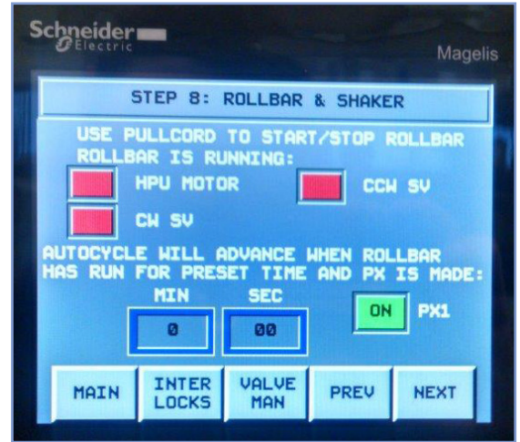
Custom Human Machine Interface Screens (HMI)
