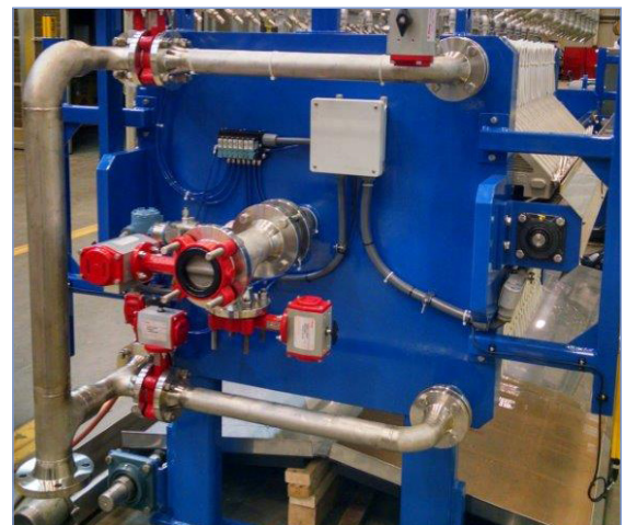
Automated Custom Process Piping Manifolds
