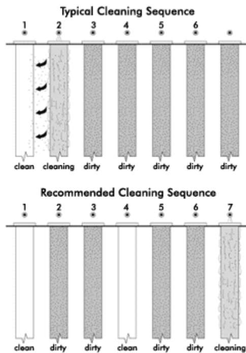
Figure 1. Recommended pulse-jet row sequencing.
